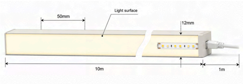
Image: Cross-sectional illustration showing the illuminated light surface, profile dimensions, and integrated LED strip arrangement.
