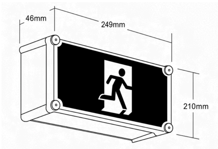
Image: Architectural dimension drawing of the exit sign
