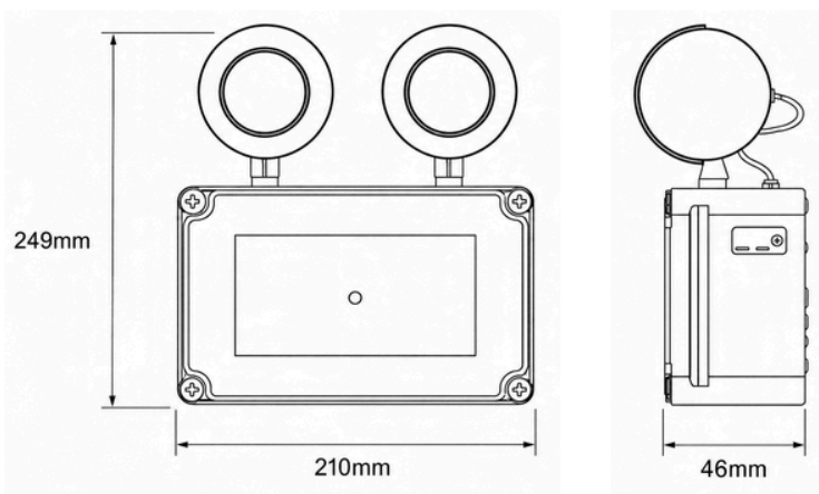
Image: Architectural dimension drawing showing the front and right-side elevations of the emergency light
