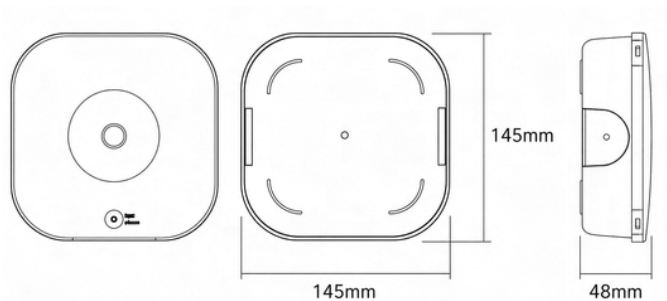
Image: Architectural dimension drawing of the emergency light
