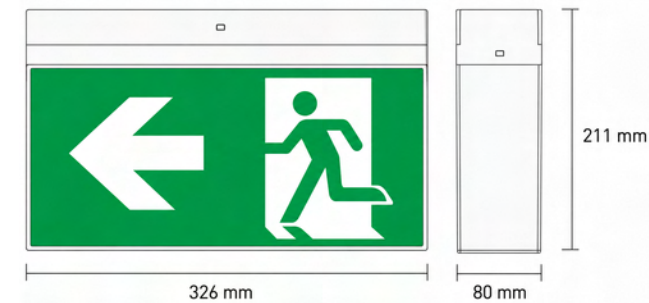
Image: Architectural dimension drawing of the exit sign
