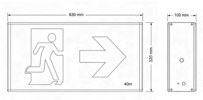
Image: Architectural dimension drawing showing the front and right-side elevations of an emergency exit sign
