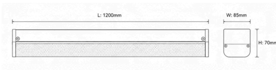
Image: dimensions of LUX BATTEN
