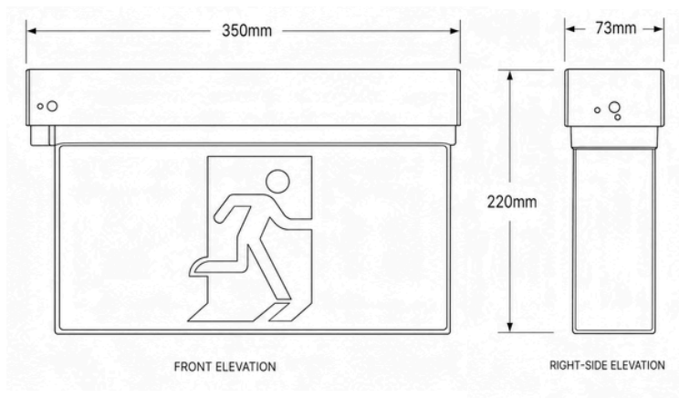
Image: Architectural dimension drawing showing the front and right-side elevations of an emergency exit sign
